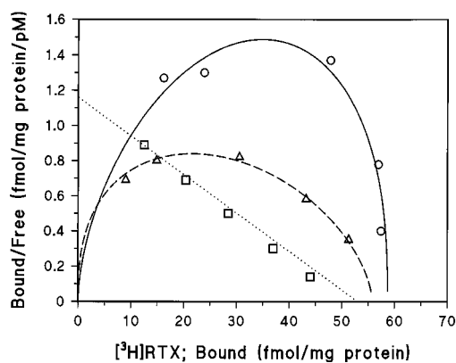
Figure 1. Scatchard plots of specific binding of [ 3 H]RTX to rat spinal cord membranes in the absence (○) or presence of 0.3 \mu\text{M} 6d (Δ) or 1.0 \mu\text{M} 6f (□). Observe that the convexity of the Scatchard plot, indicative of positive cooperative binding, is diminished in the presence of 6d and completely abolished (linear plot) in the presence of 6f . The experiments shown are representative. For binding parameters (average \pm SEM), see Table 1.
